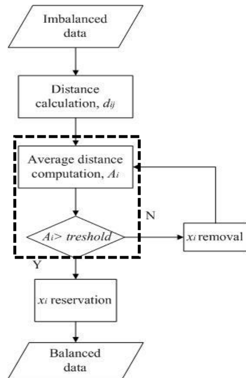
Figure 4. Flowchart of Distance-based Undersampling Technique (Li et al., 2013)
