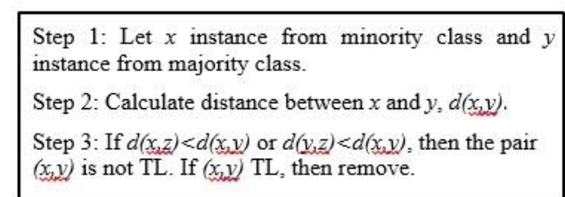
Figure 1. Algorithm of Tomek Links
