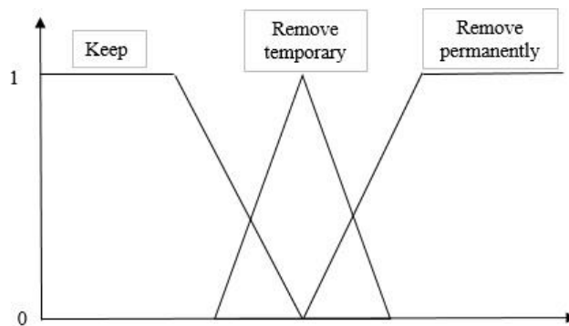
Figure 7. Triangular and Trapezoidal Membership Function
