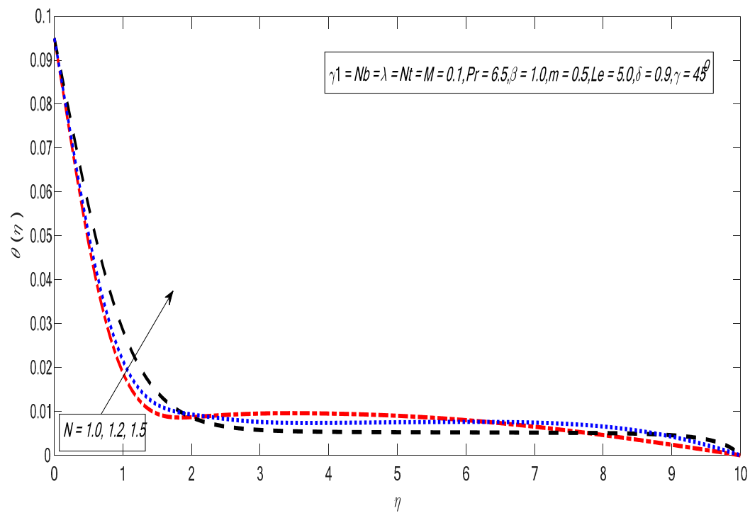
Figure 12. Variations in temperature profile for several values of N .
