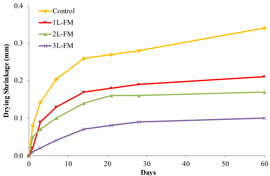
Fig. 6. Drying shrinkage of 1000 kg/m³ density LFC confined with varying layers of fibreglass fabric
