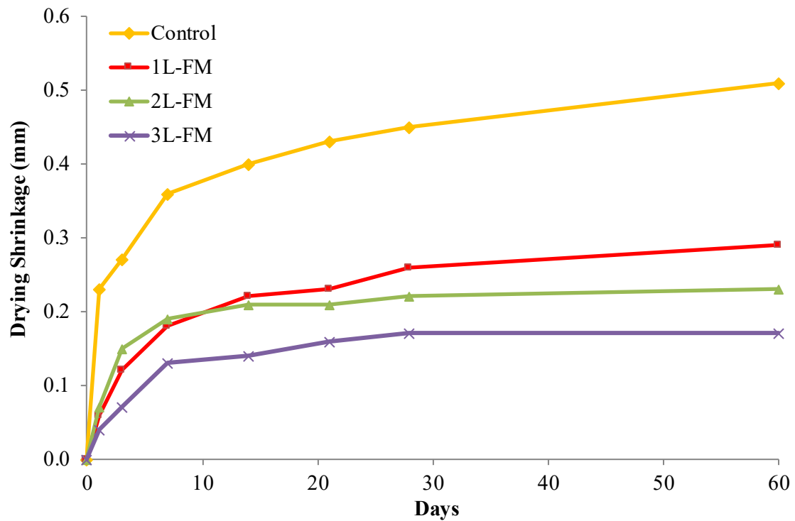
Fig. 5. Drying shrinkage of 500 kg/m³ density LFC confined with varying layers of fibreglass fabric
