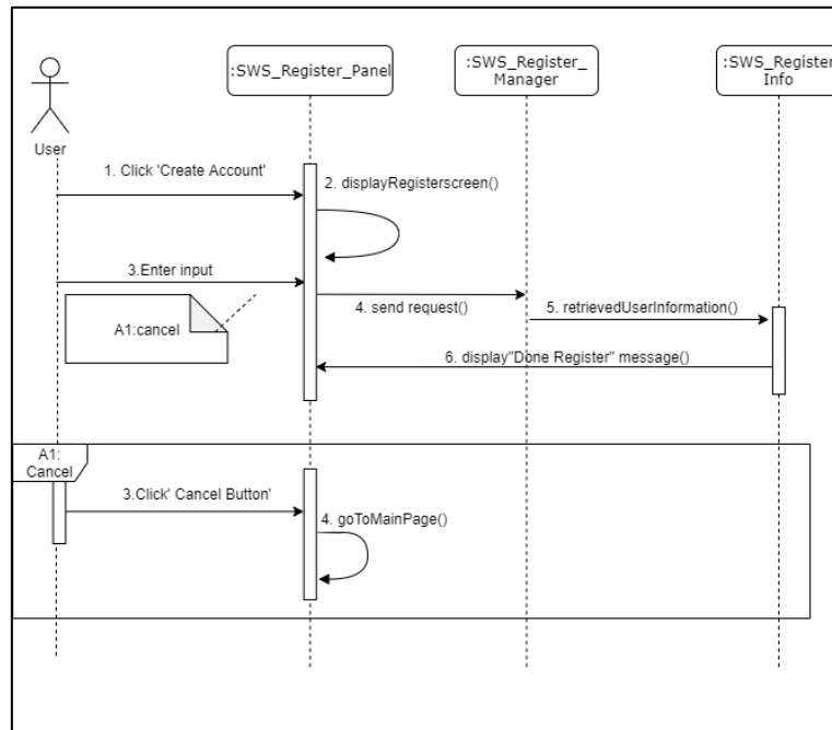
Sequence diagram of Register
