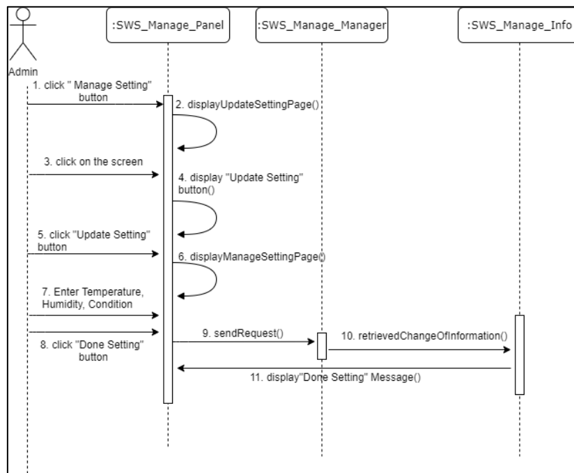
Sequence diagram of Manage Setting
