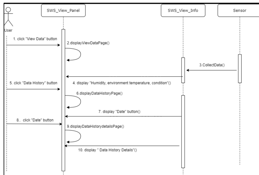
Sequence Diagram of View Data
