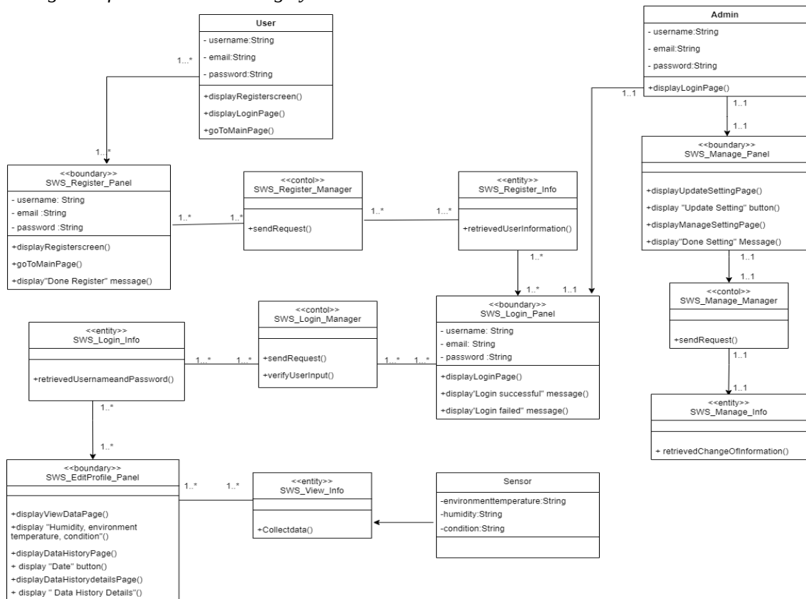
Class diagram of IoT Smart Watering System
