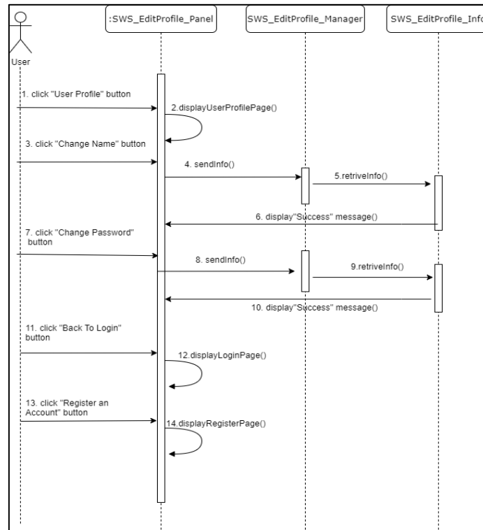
Sequence Diagram of Edit Profile
