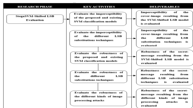
Figure 2. StegaSVM-Shifted LSB Evaluation Phase
